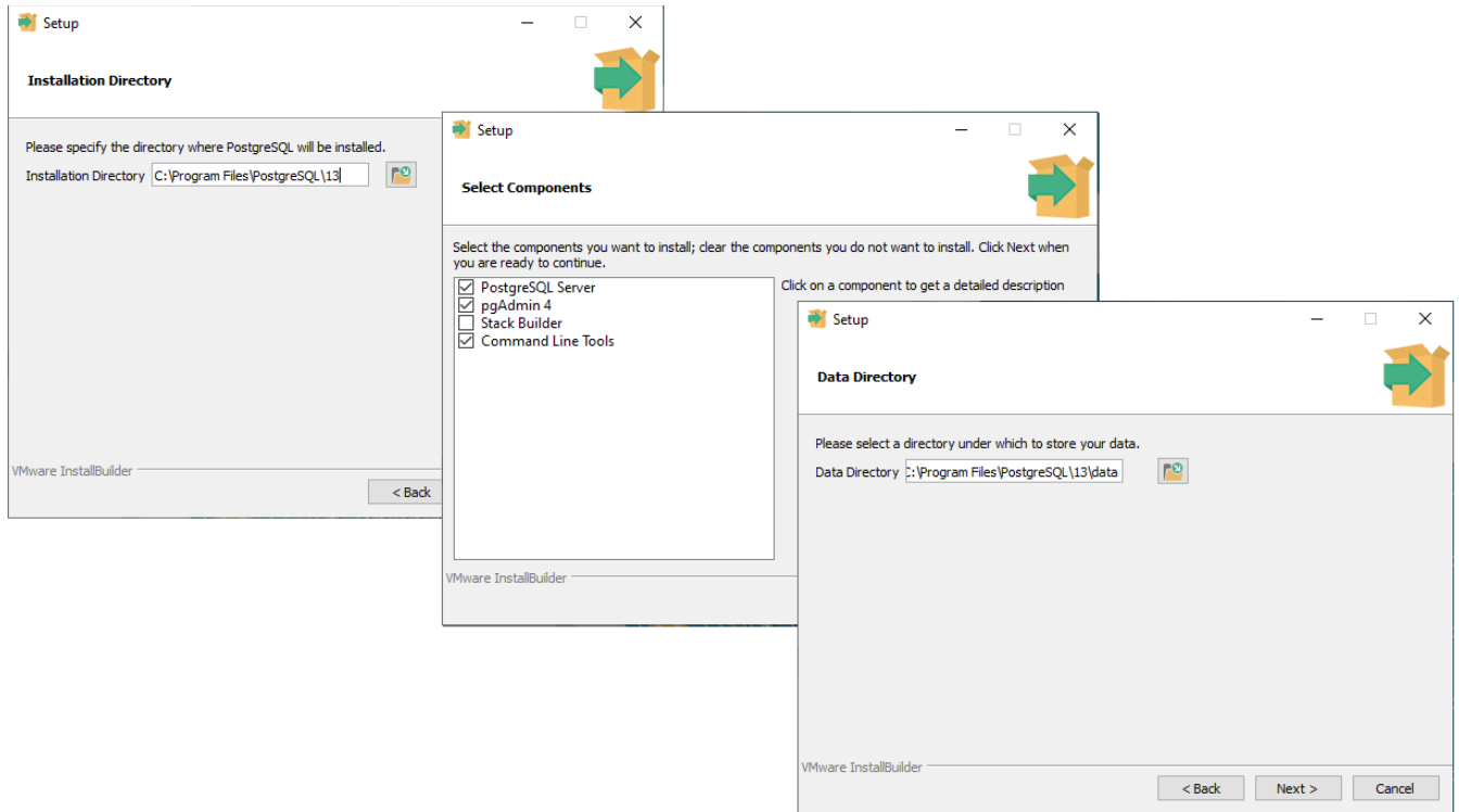
Figure 3. Selection of folders where the PostgreSQL should be installed and data stored
