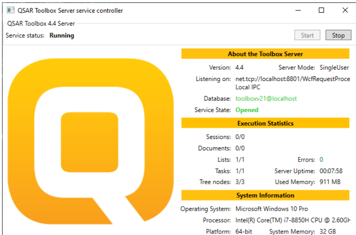
Figure 2: Service UI
